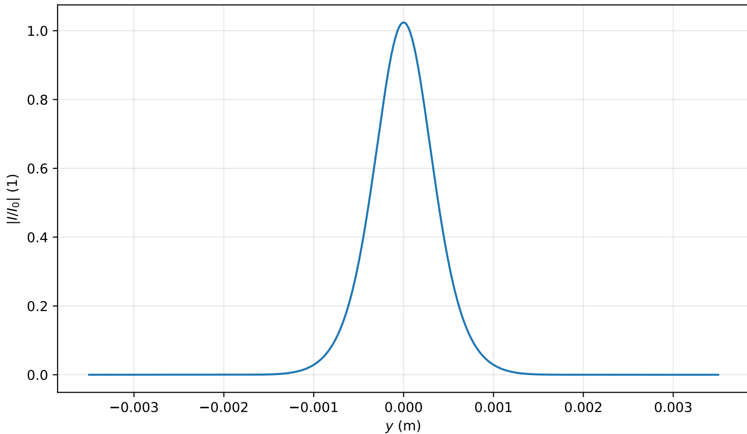
Intensity profile I(x=0, y, z=1.194)/I_0 , \text{Pin}=0.5\text{Pcr} , artificial time
